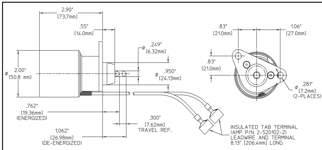
Figure 1. Two-Hole Flange Push Type Actuator
