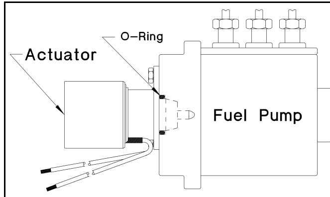
Figure 2. Mounting of 0200 Actuator to Fuel Pump
